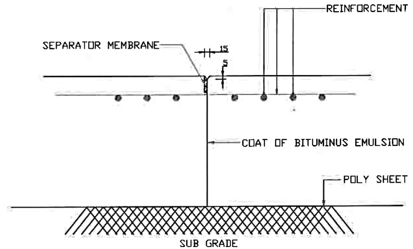
DETAILS "B" (CONTRACTION JOINT)
