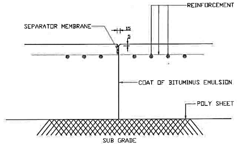
DETAILS "B" (CONTRACTION JOINT)
