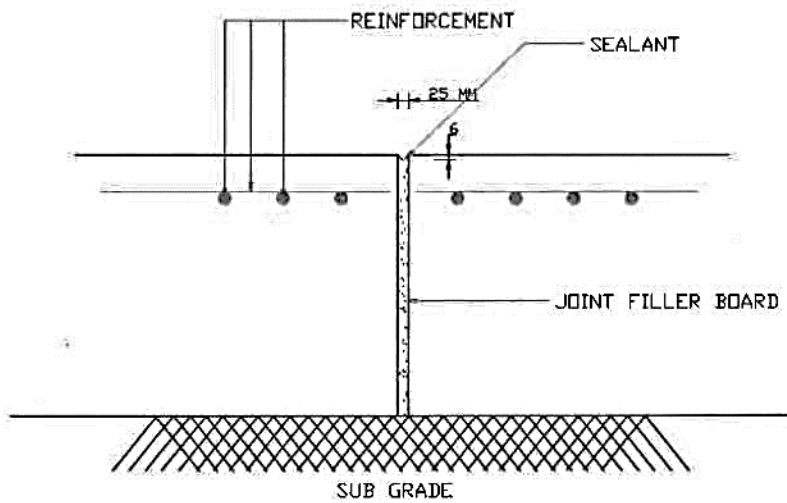
DETAILS "A" (EXPANSION JOINT)
