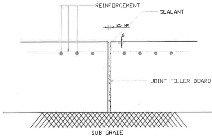
DETAILS "A" (EXPANSION JOINT)
