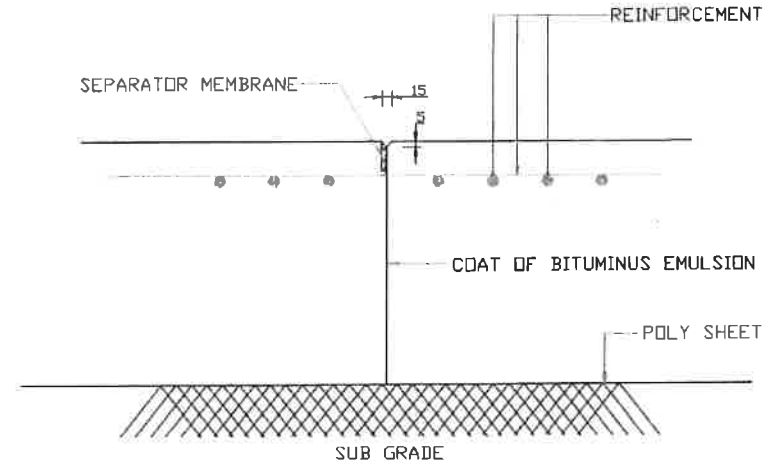
DETAILS "B" (CONTRACTION JOINT)
